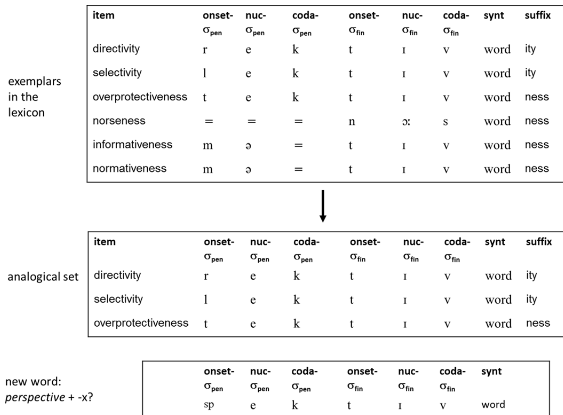
Figure 8 The general architecture of an analogical model
