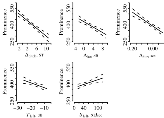
Figure 2: Partial effects of a linear regression model predicting prominence ratings.
